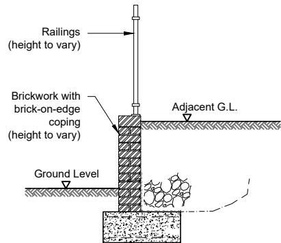
Typical Railings & Retaining Wall Detail
