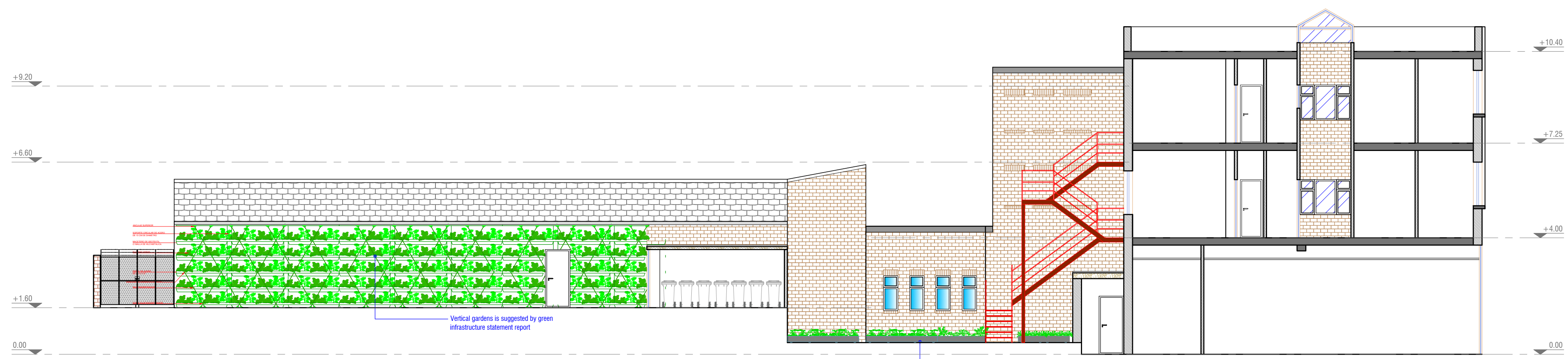
Section B''-B'' Proposed green infrastructure of vertical gardens and plant pots
