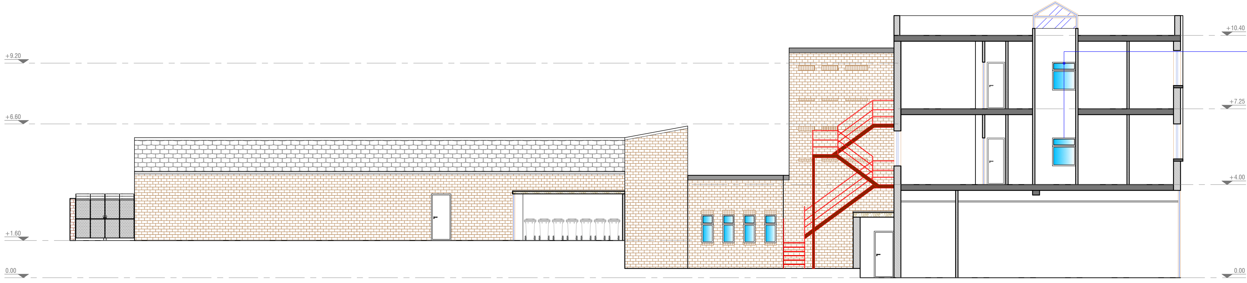
Side view B-B, Proposed
