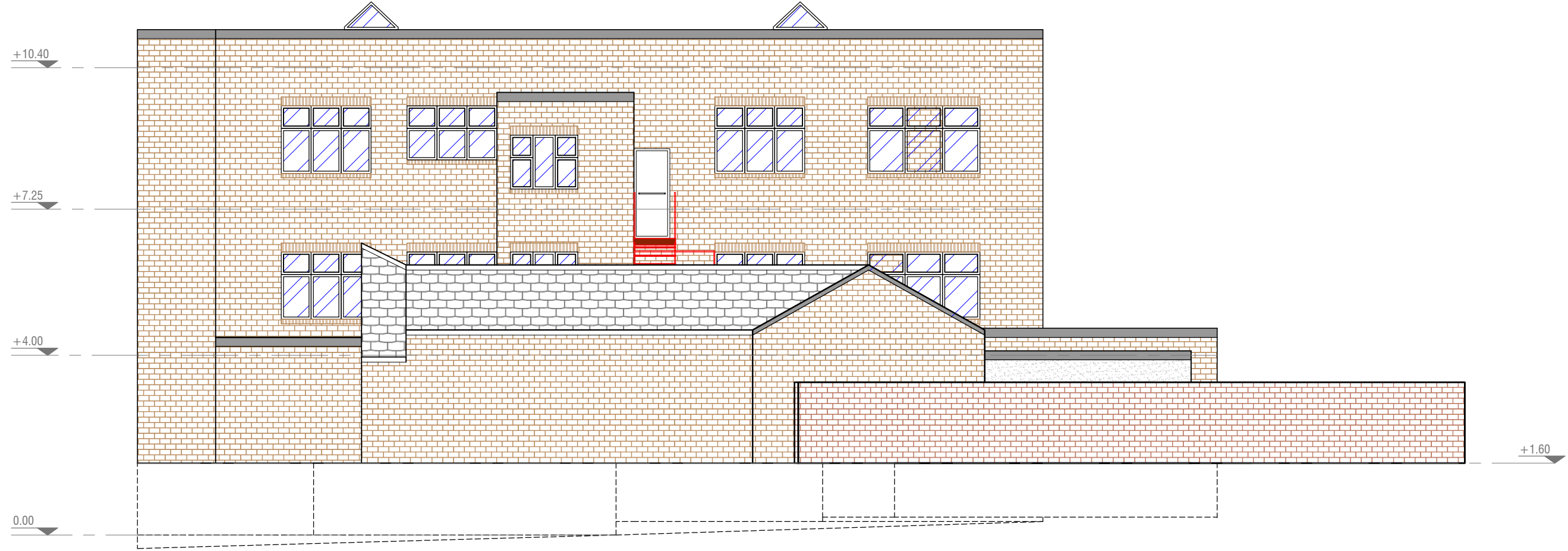
Rear view - East, Proposed
