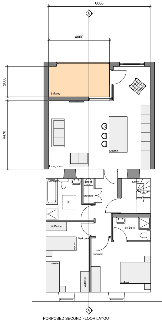
PORPOSED SECOND FLOOR LAYOUT
