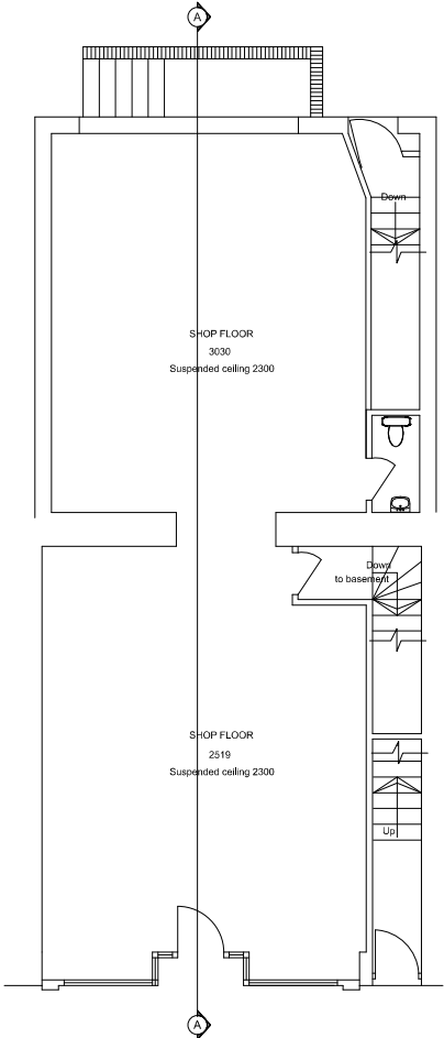
EXISTING & PROPOSED GROUND FLOOR LAYOUT
