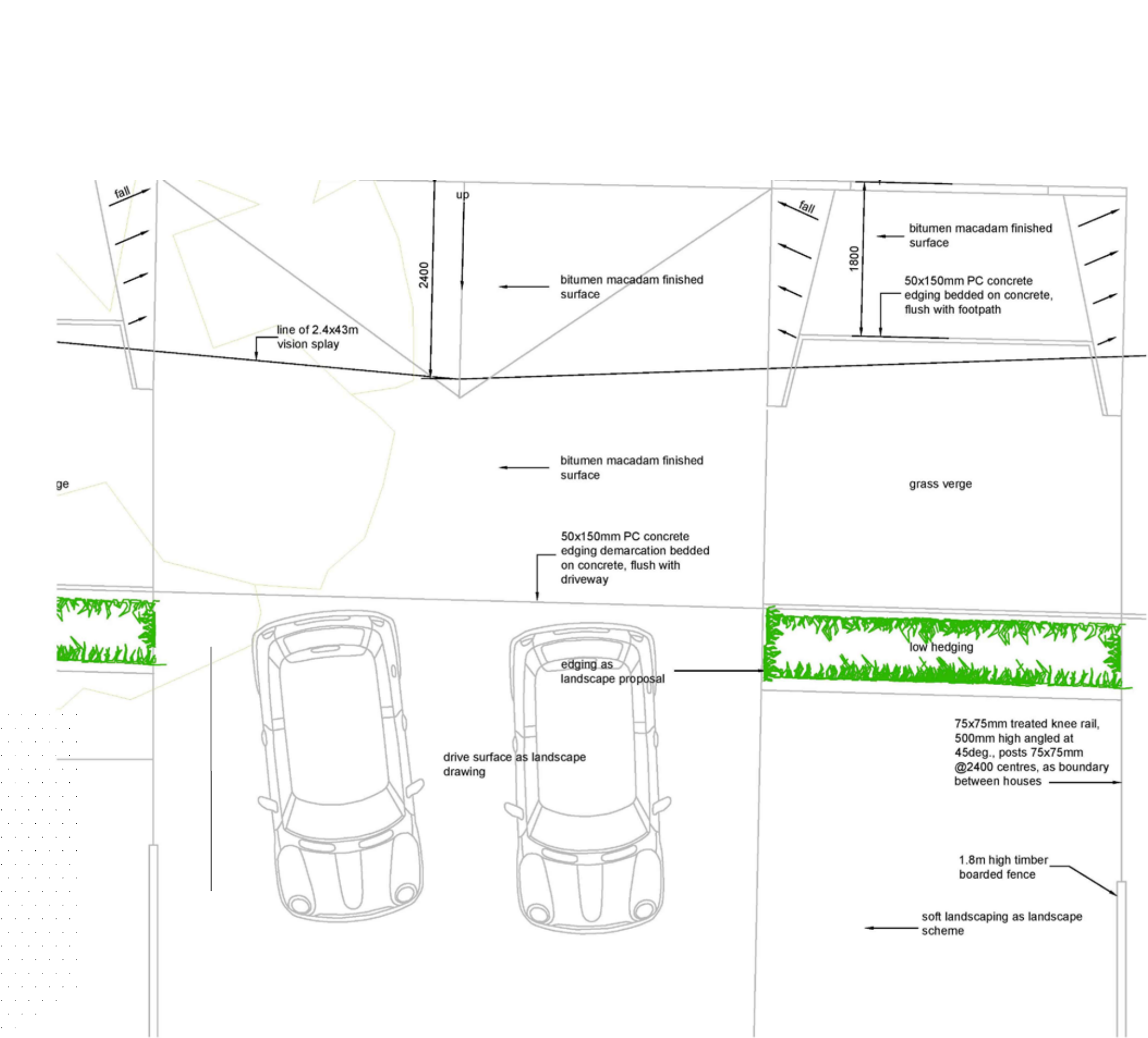
Typical Crossover/ Plan Scale 1:50
