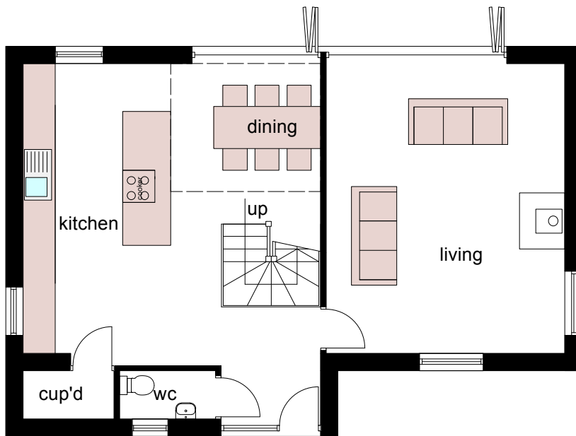
GROUND FLOOR PLAN 61sqm
