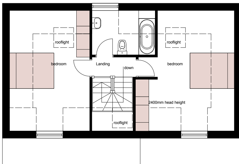
FIRST FLOOR PLAN - 55sqm
