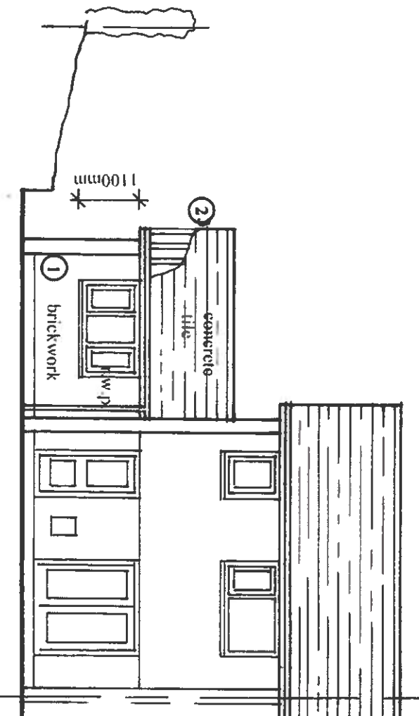
FRONT ELEVATION (1:100)
