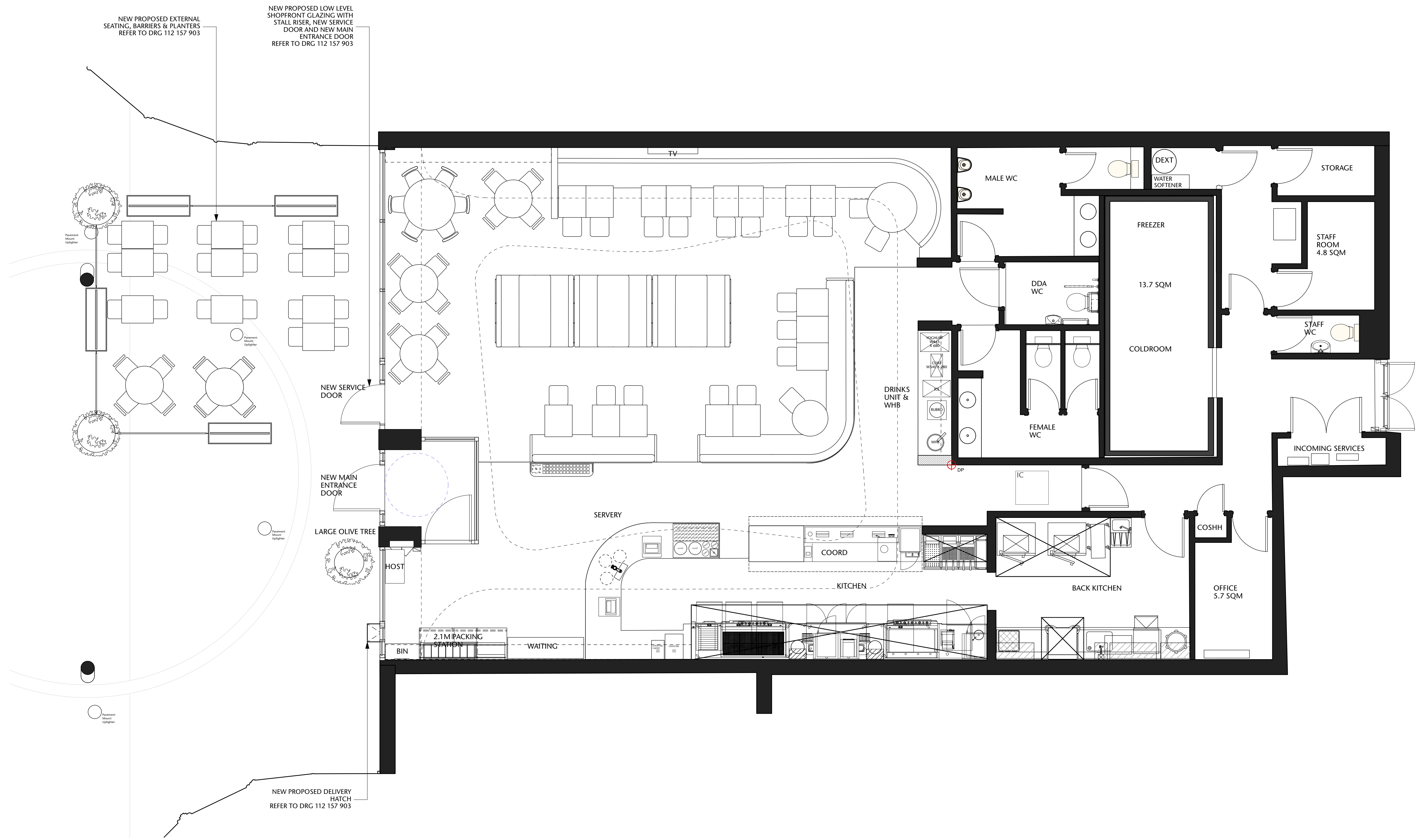
01 PROPOSED GENERAL ARRANGEMENT PLAN SCALE 1:50@A1
