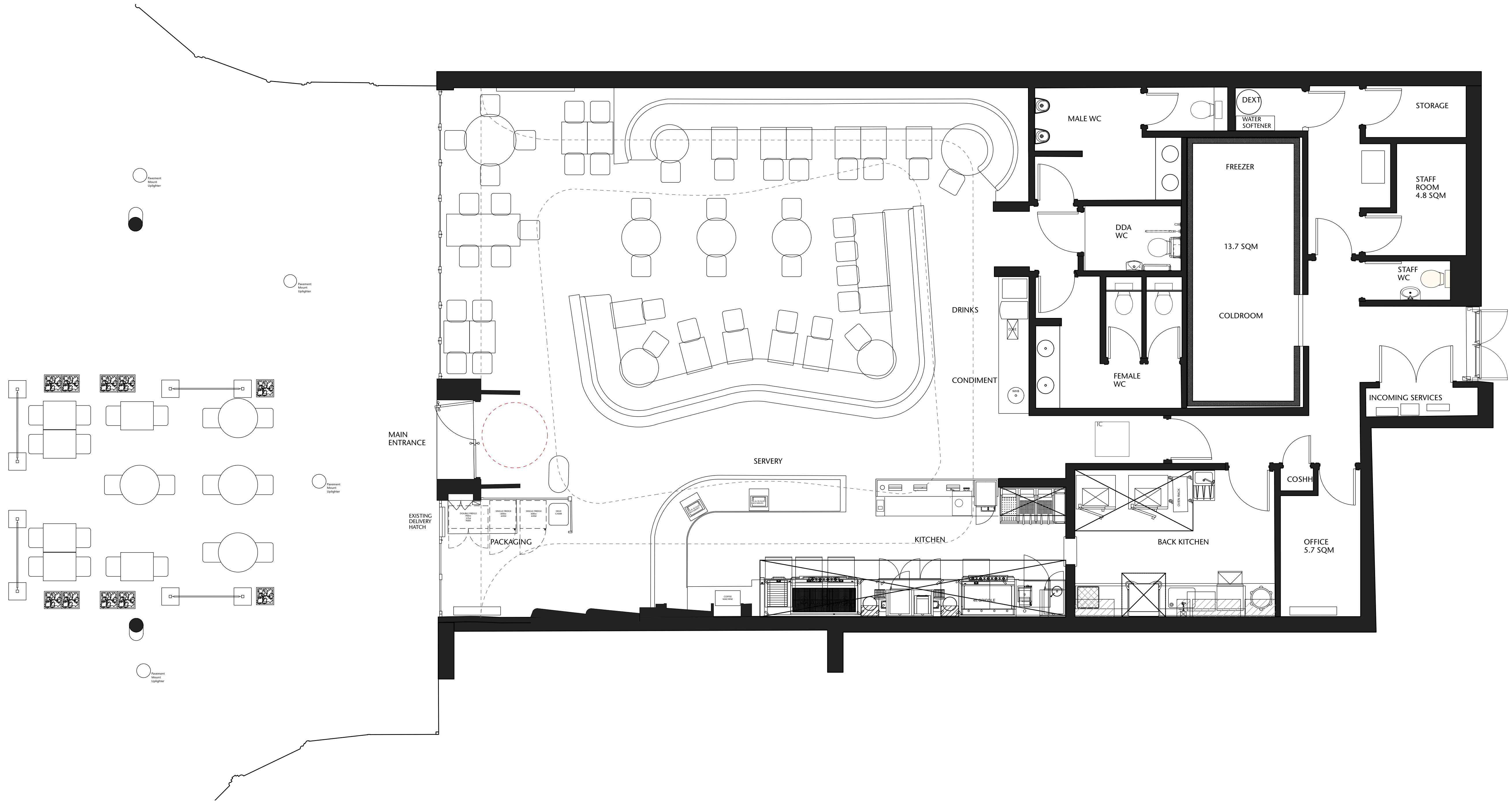
01 EXISTING GENERAL ARRANGEMENT PLAN SCALE 1:50@A1
