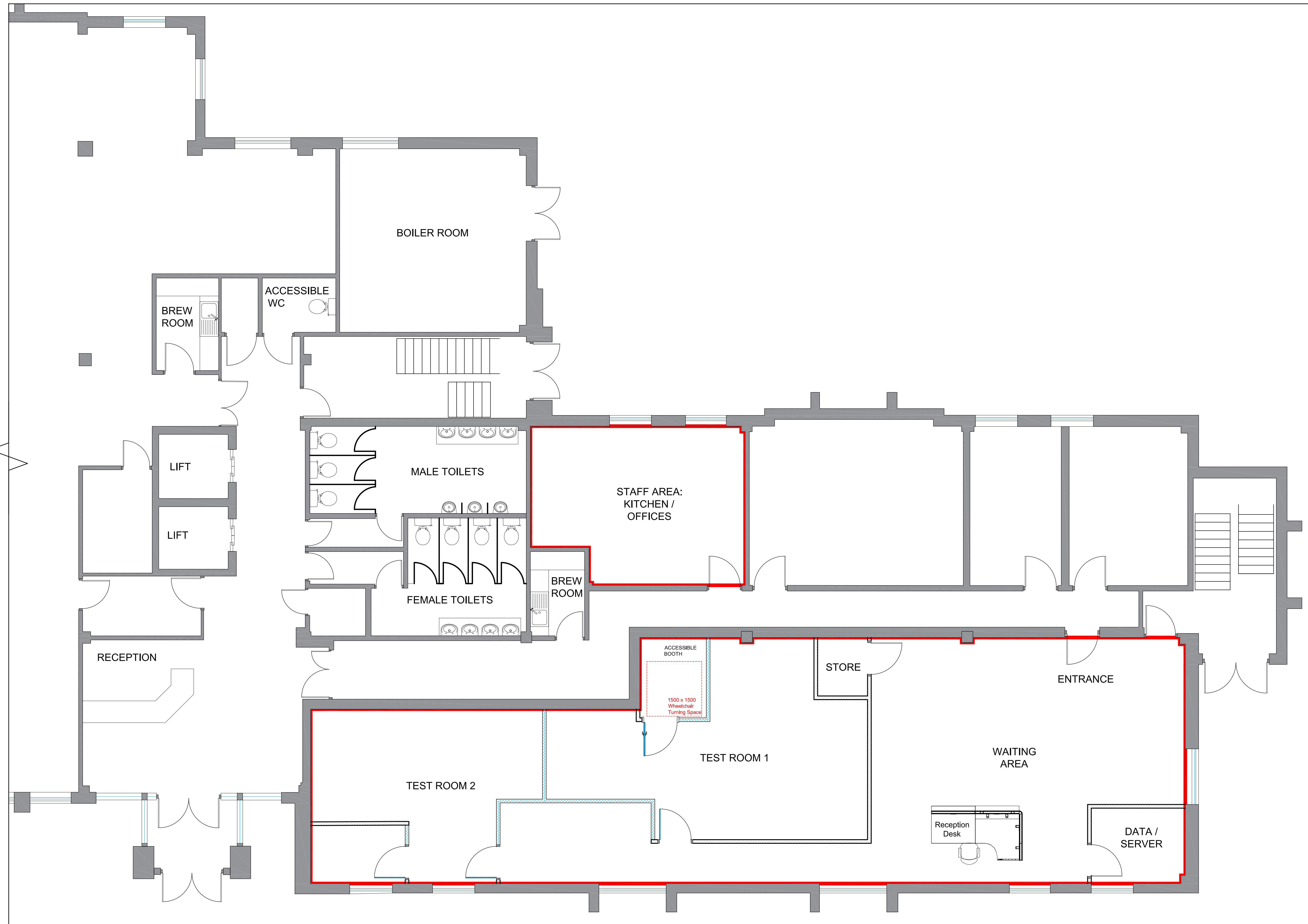
Merthyr Tydfil PPC - Proposed GA Plan - Ground Floor Scale 1:50 @ A1
