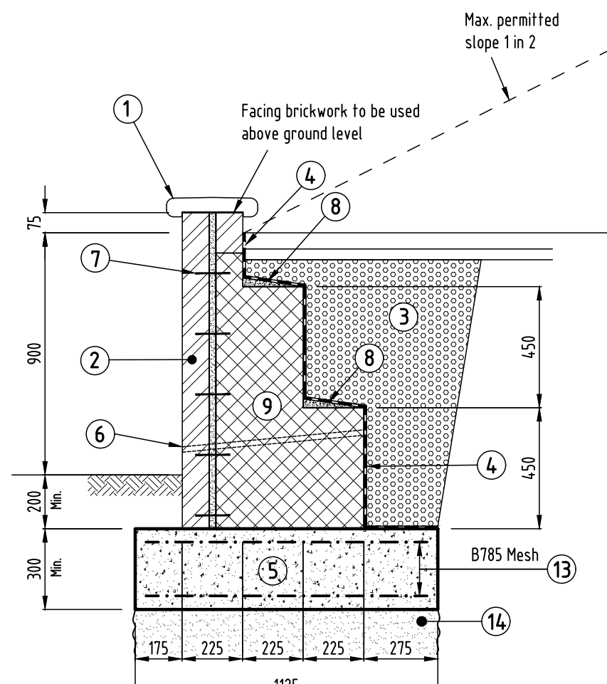
Type 'C1' Retaining Wall:- Max. retained height 0.90m. Scale 1:20
