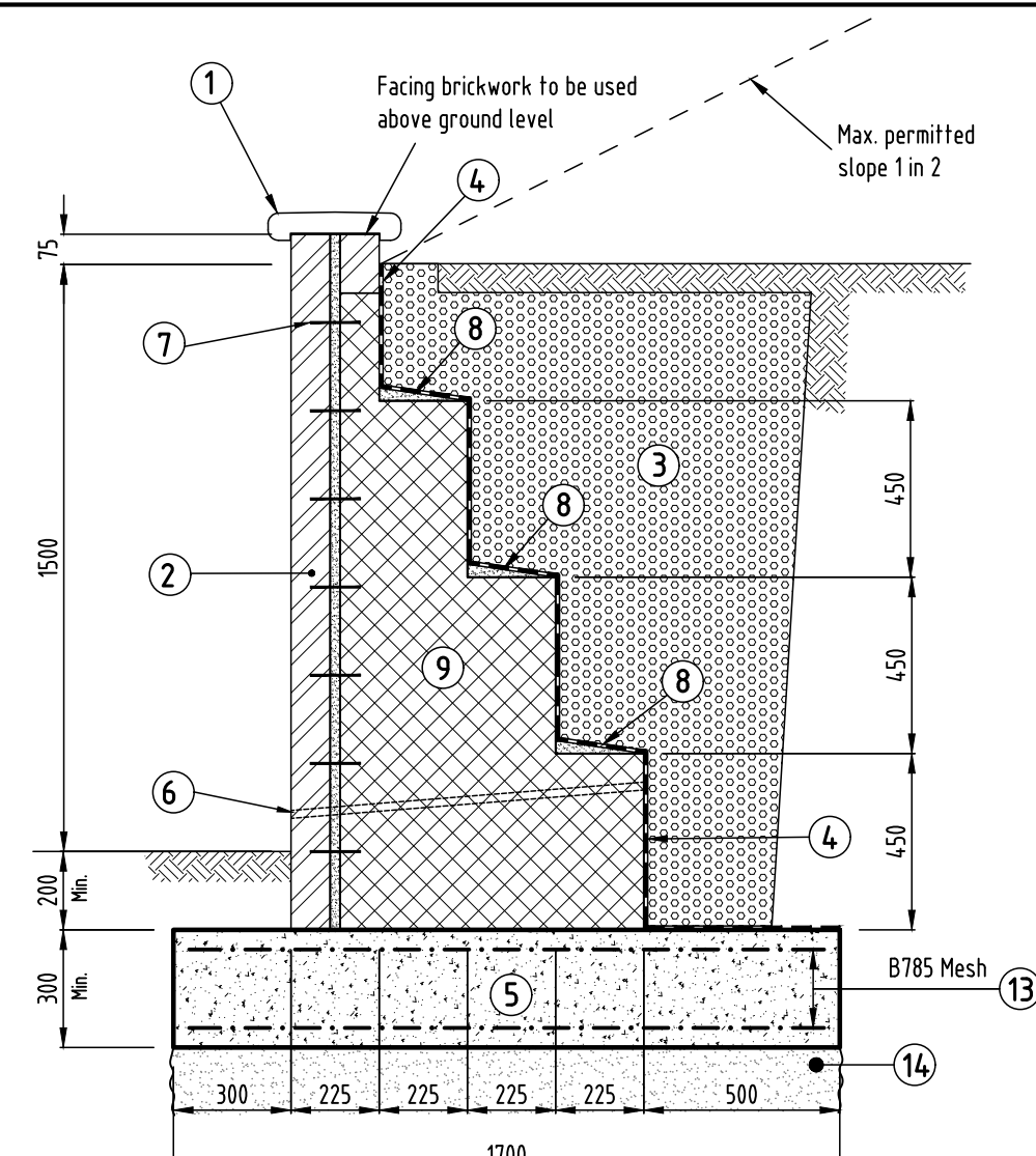
Type 'E1' Retaining Wall:- Max. retained height 1.50m. Scale 1:20
