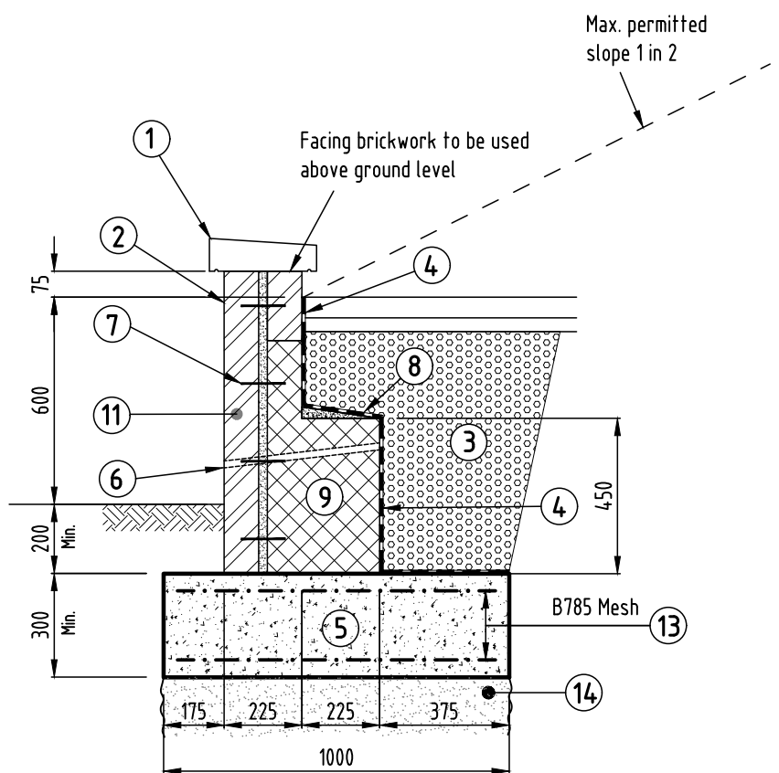
Type 'B1' Retaining Wall:- Max. retained height 0.60m. Scale 1:20
