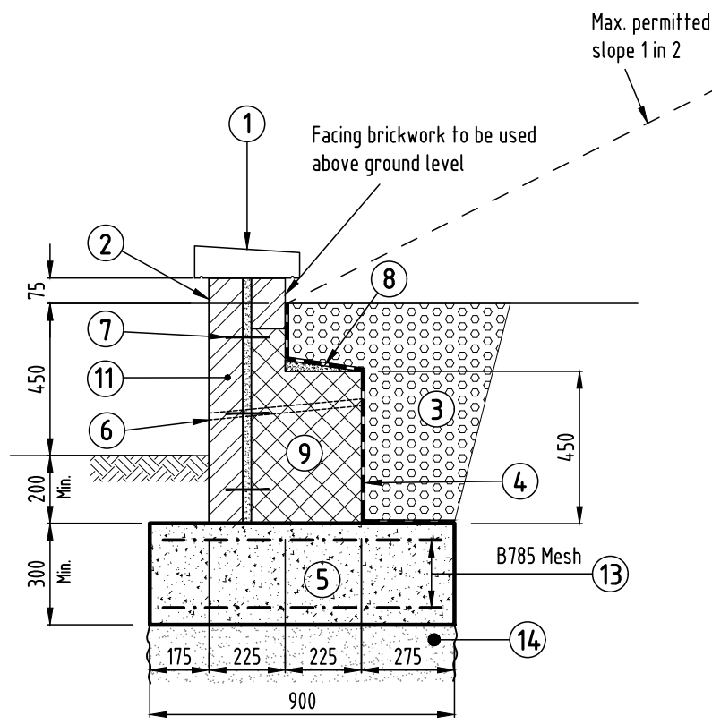
Type 'A1' Retaining Wall:- Max. retained height 0.45m. Scale 1:20
