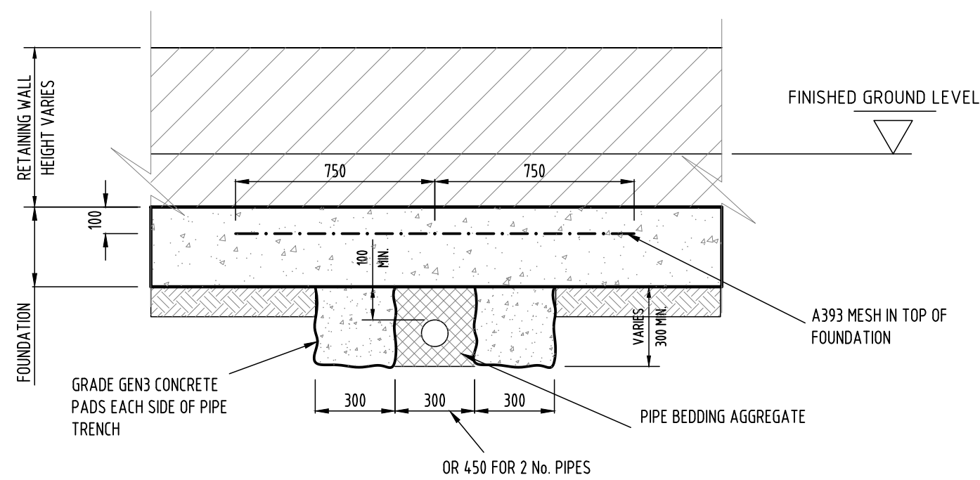
Detail for Sewers Passing under Retaining Wall: Elevation on Retaining Wall. Scale 1:20
