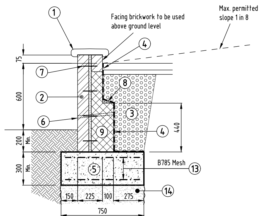
Type 'B' Retaining Wall:- Max. retained height 0.60m. Scale 1:20
