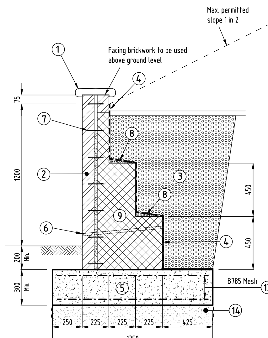
Type 'D1' Retaining Wall:- Max. retained height 1.20m. Scale 1:20
