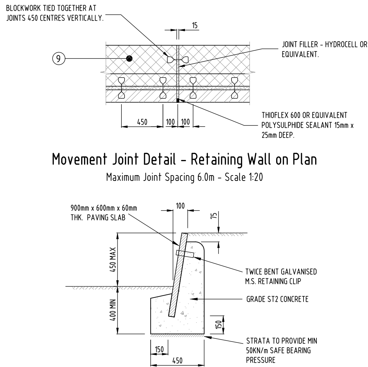
Paving Slab on Edge : Retaining Wall Detail for Garden Areas only up to 450mm Max.
