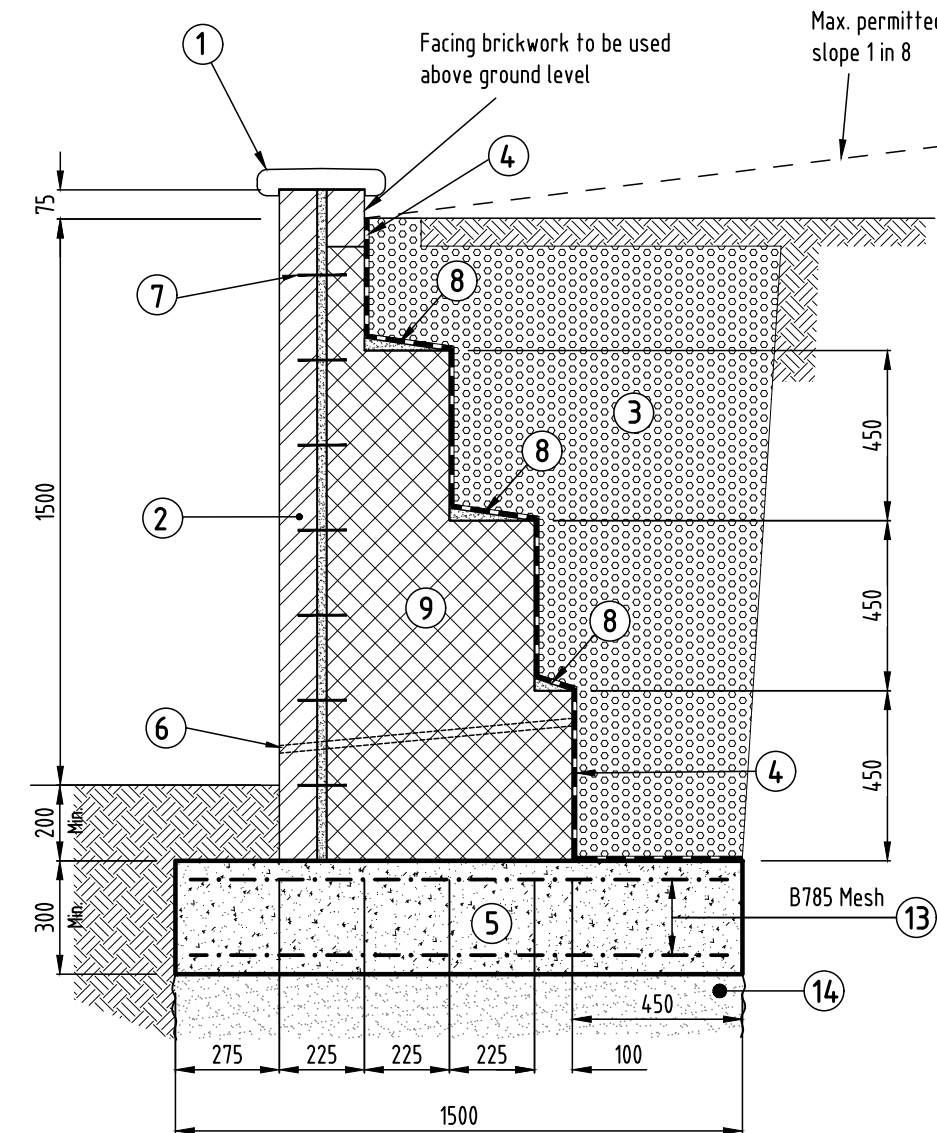
Type 'E' Retaining Wall:- Max. retained height 1.50m. Scale 1:20
