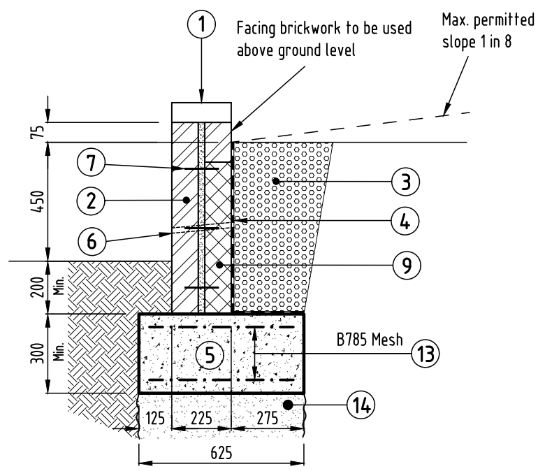
Type 'A' Retaining Wall:- Max. retained height 0.45m. Scale 1:20
