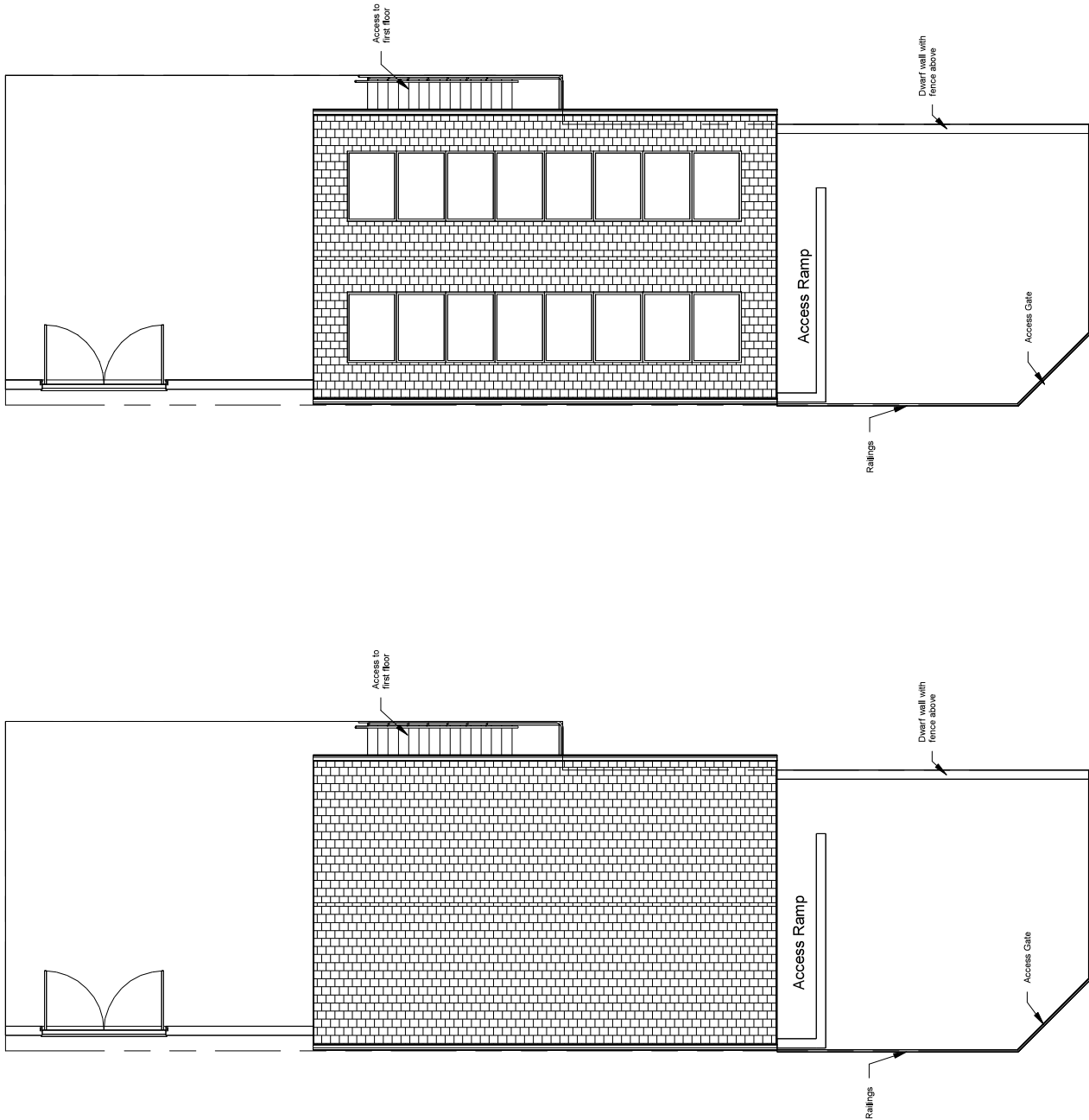
2 Proposed Site 1 : 100
