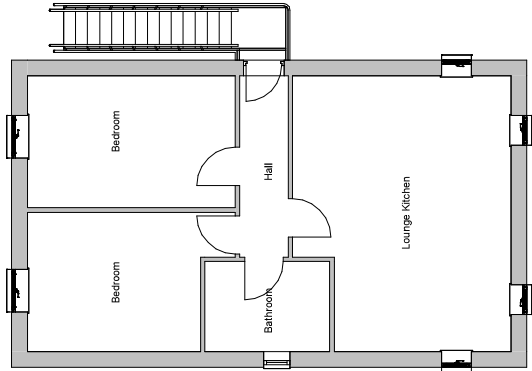
2 Proposed First Floor 1 : 100
