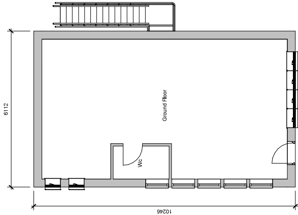
1 Proposed Ground Floor 1 : 100
