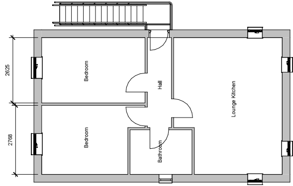
2 Existing First Floor 1 : 100
