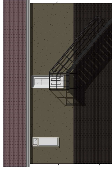
6 Existing Side 2 Elevation 1 : 100
