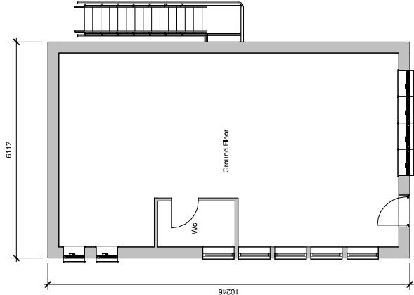
1 Existing Ground Floor 1 : 100
