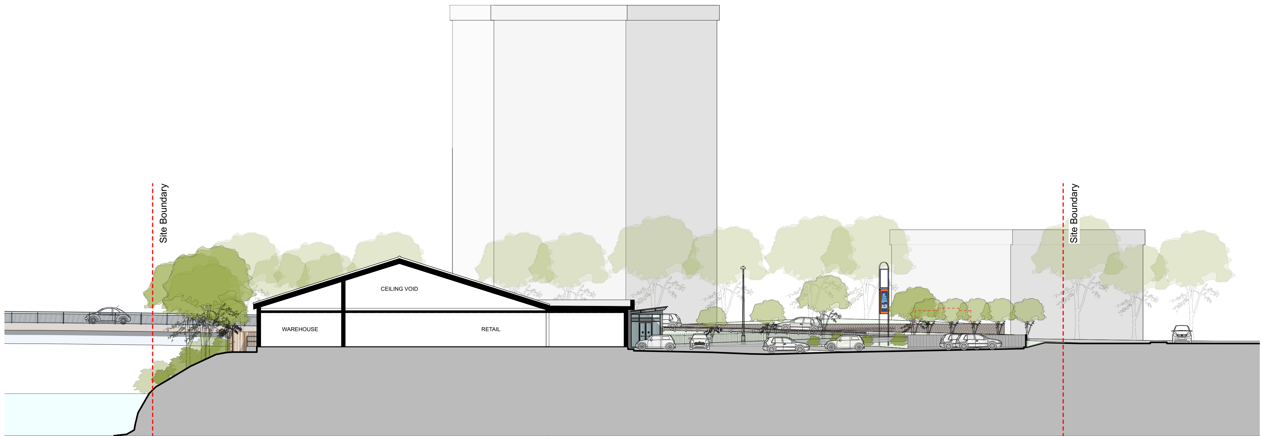
PROPOSED CAR PARK SECTION A-A
