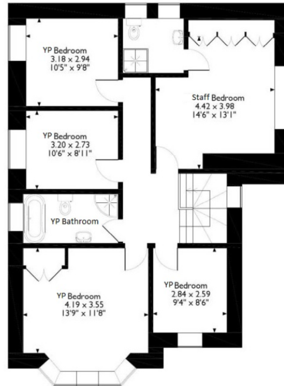
First Floor
