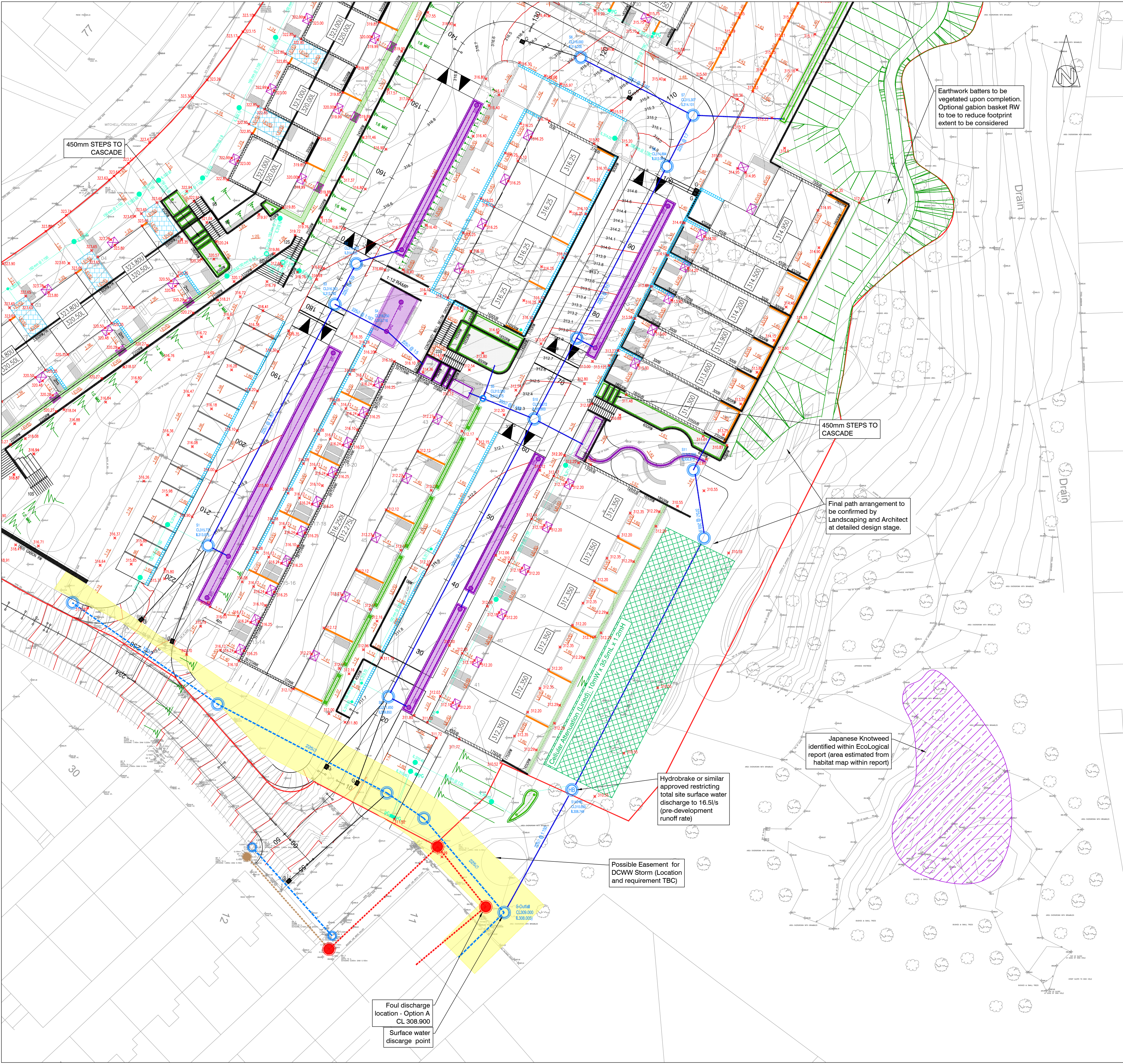
SITE LOCATION PLAN - NTS
