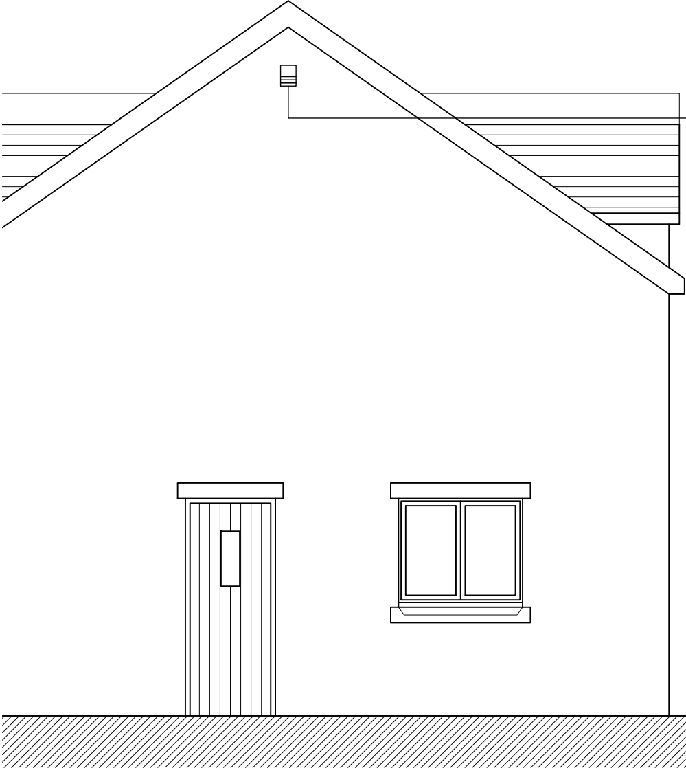
PROPOSED SIDE ELEVATION facing angus street
