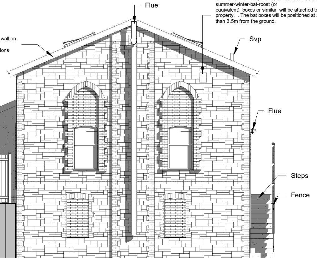
2 Proposed Rear Elevation 1 : 100
