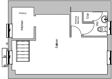
2 Existing First Floor 1 : 100
