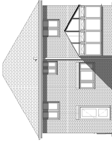
4 Existing Rear Elevation 1 : 100
