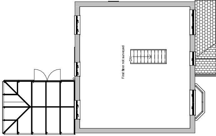
2 Existing First Floor 1 : 100
