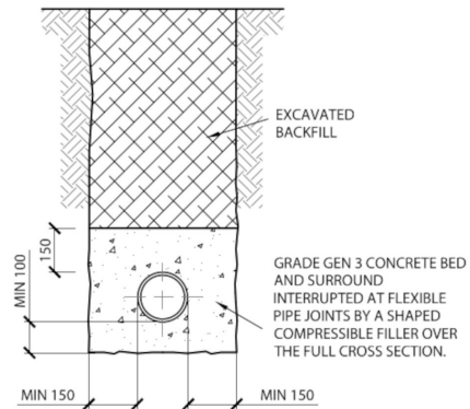
DETAIL 1:20 2 CLASS 'Z' CONCRETE SURROUND
