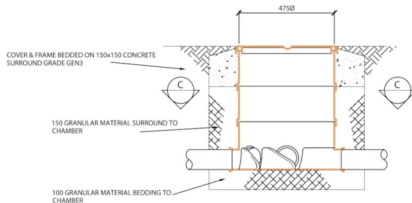
DETAIL 1:20 6 TYPICAL POLYPROPYLENE INSPECTION CHAMBER
