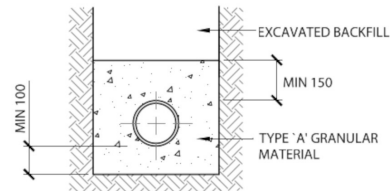
DETAIL 1:20 4 CLASS 'N' BEDDING
