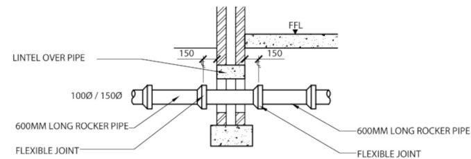
DETAIL 1:20 5 PENETRATION THROUGH EXISTING WALL
