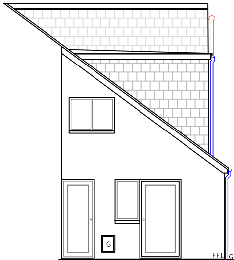
Proposed Front Elevation 1:100 As Existing
