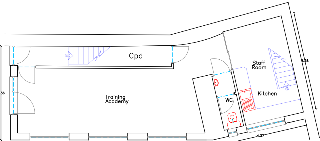
Proposed GF Plan 1:100 As Existing
