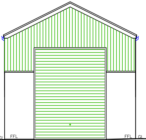
Proposed Front Elevation 1:100 As Existing
