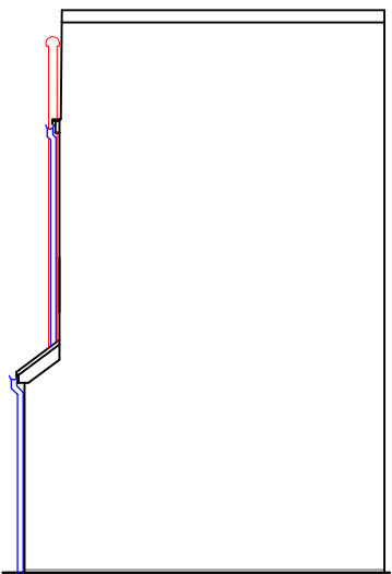
Proposed Rear Elevation 1:100 As Existing
