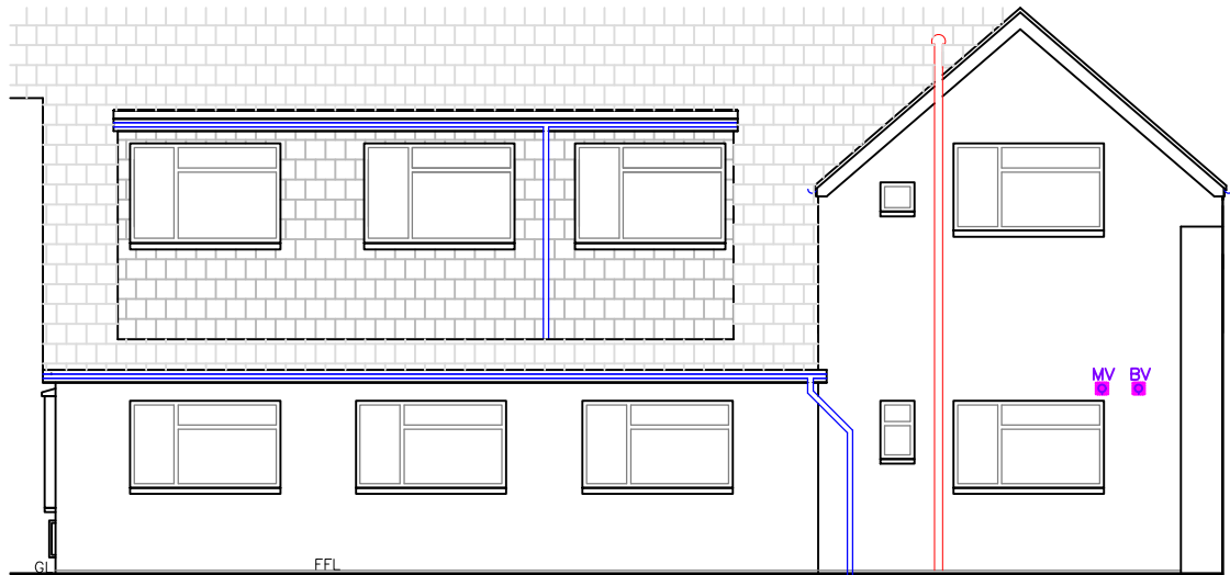
Proposed Side Elevation 1:100 As Existing
