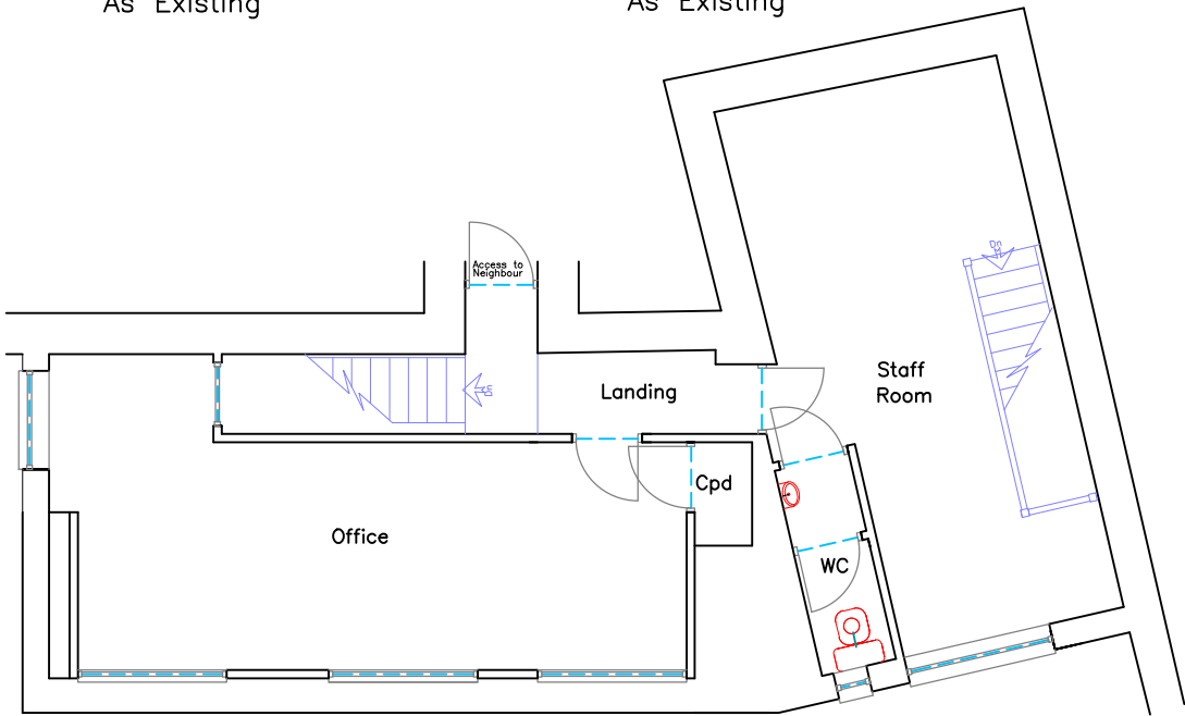
Proposed FF Plan 1:100 As Existing
