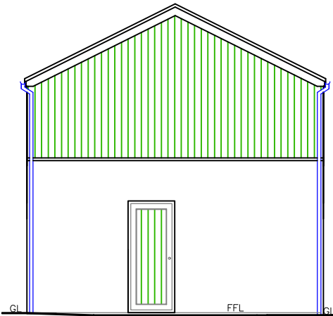
Proposed Rear Elevation 1:100 As Existing
