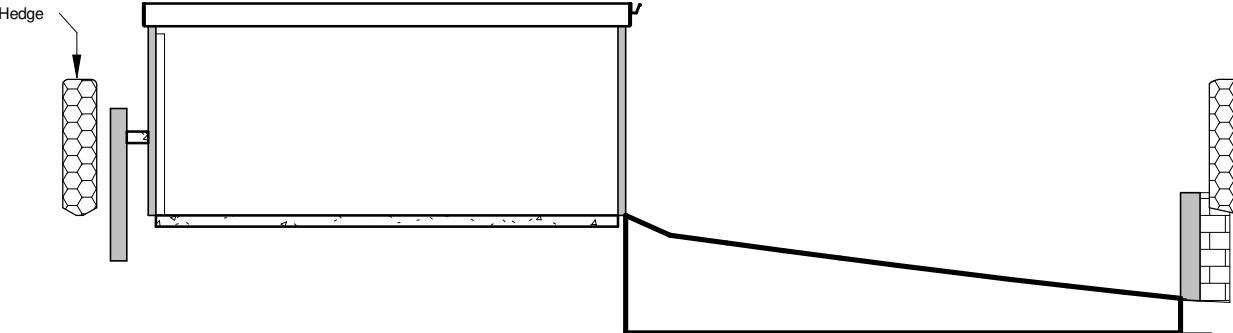
4 Proposed Section B 1 : 100
