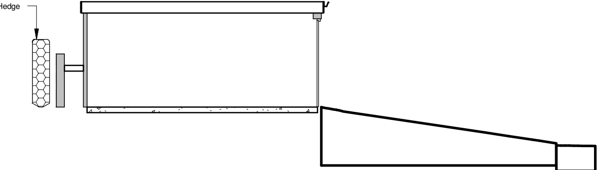
3 Proposed Section A 1 : 100
