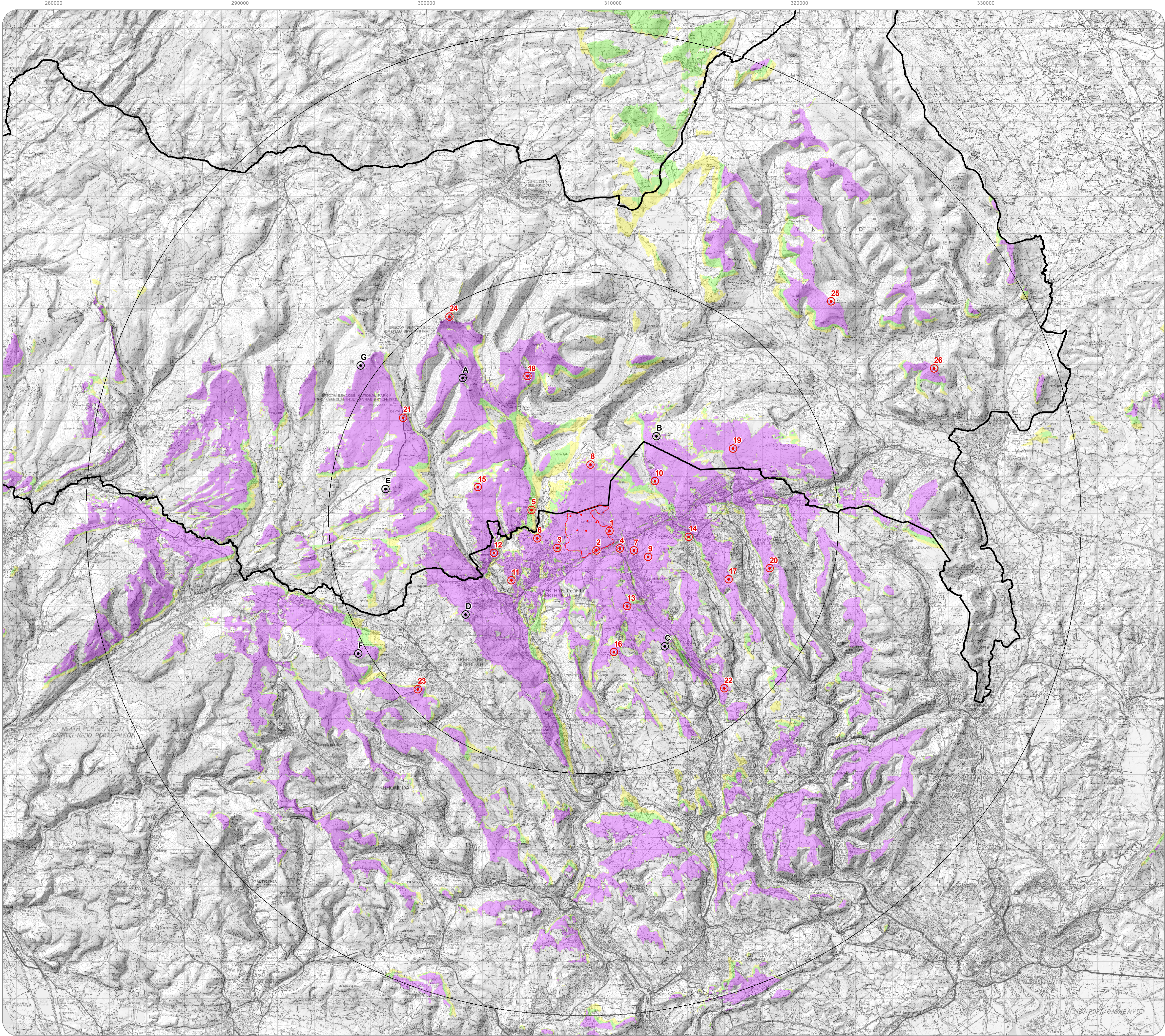
Figure 5.11b Blade Tip ZTV with Viewpoints
