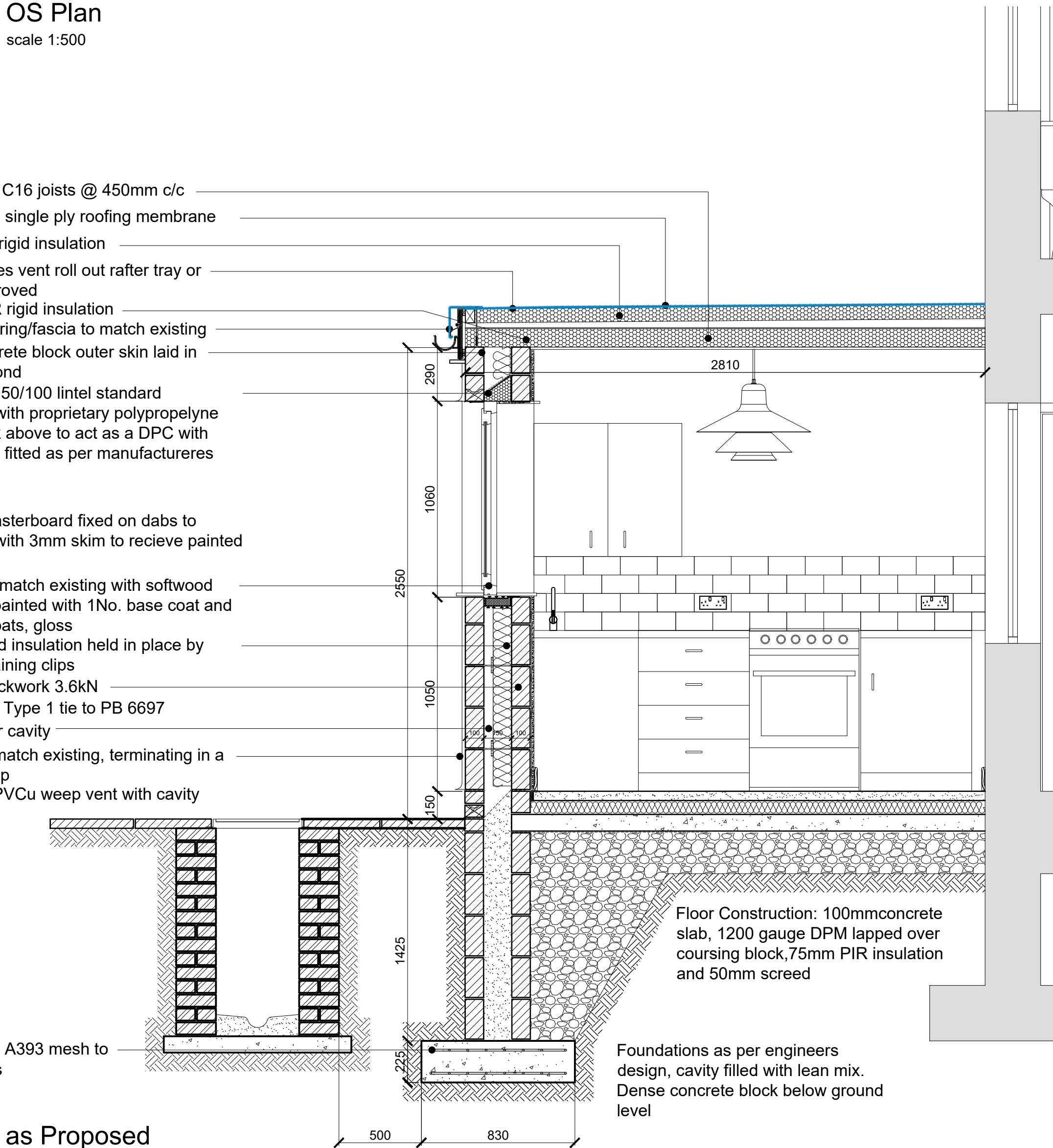
Section as Proposed scale 1:20
