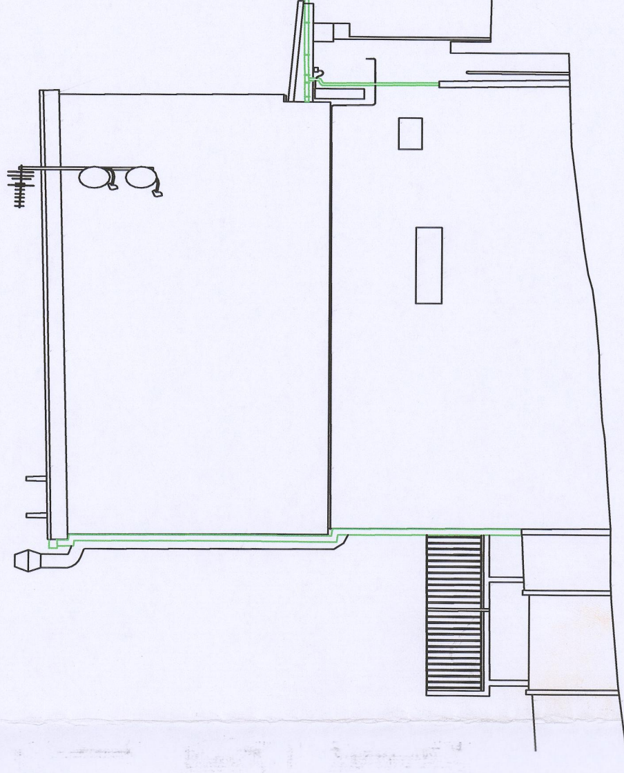
South Elevation
