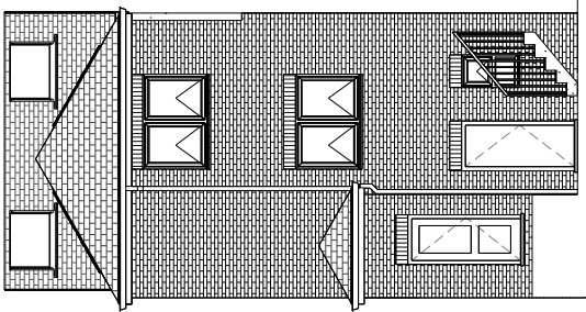
2 Proposed Rear Elevation 1 : 100
