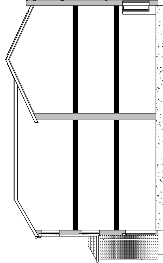
4 Proposed Section 1 : 100
