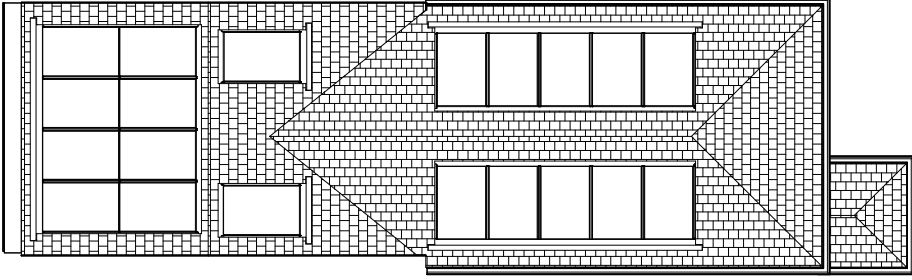
4 Proposed Site 1 : 100
