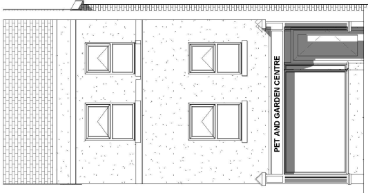
① Existing Front Elevation 1 : 100
