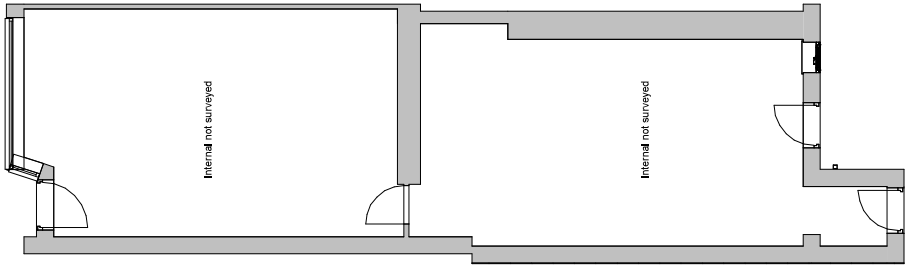
1 Existing Ground Floor 1 : 100
