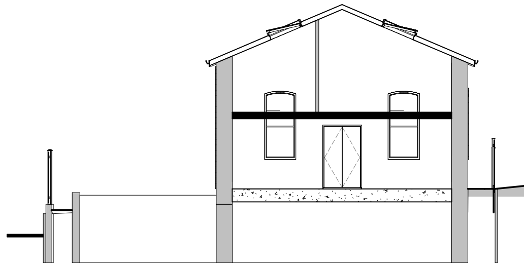
(B) Proposed Section B 1 : 100
