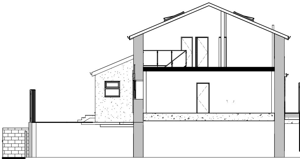
(A) Proposed Section A 1 : 100
