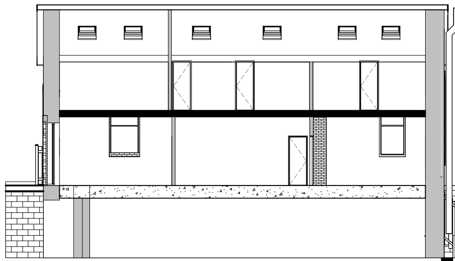
(C) Proposed Section C 1 : 100
