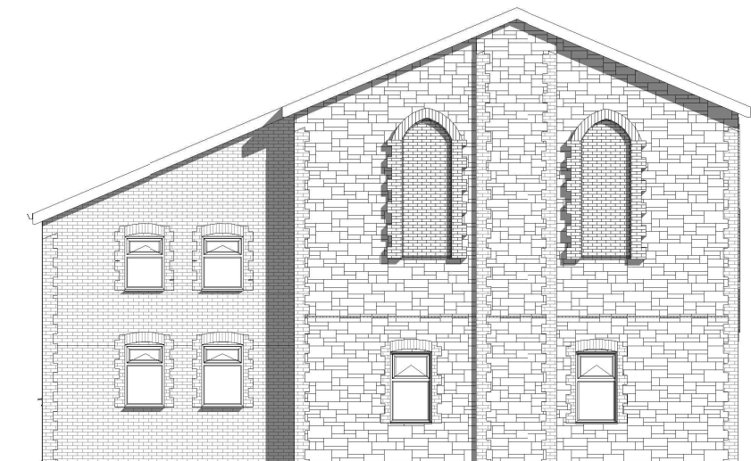
2 Existing Rear Elevation 1 : 100
