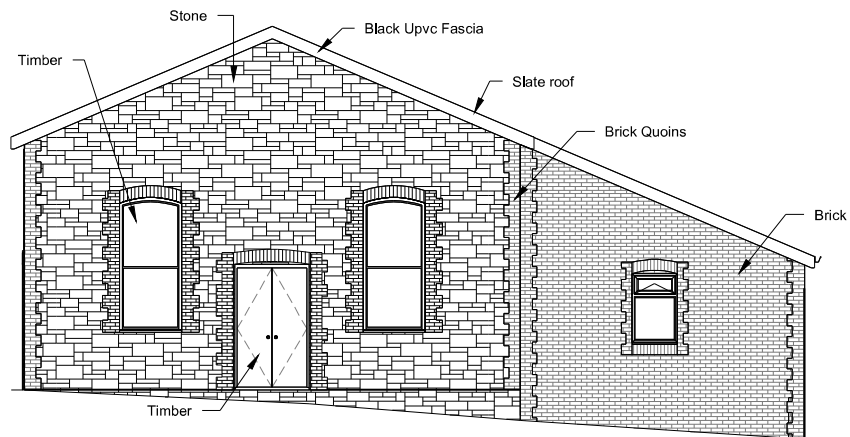
1 Existing Front Elevation 1 : 100
