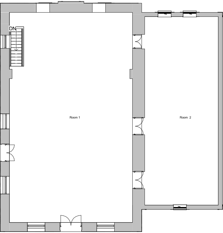
① Existing Ground Floor 1 : 100
