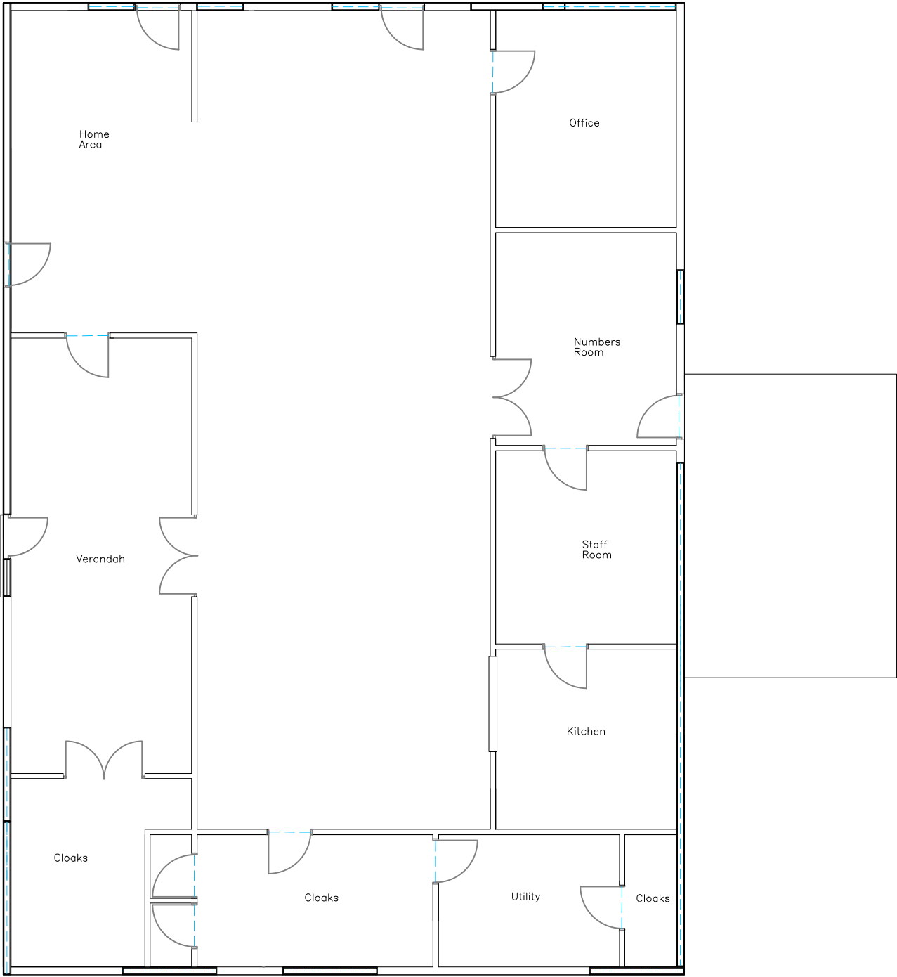
Existing Floor Plan 1:100
