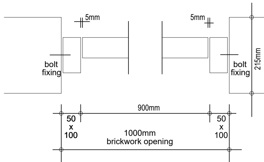
PLAN DETAIL 02
