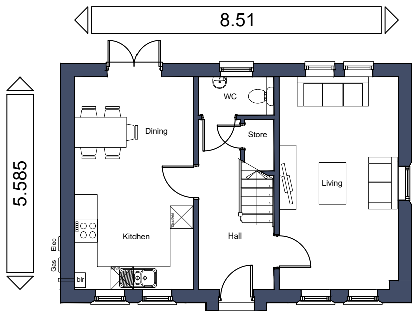
Ground Floor Plan Opp Plots 1, 86, 97, 112
