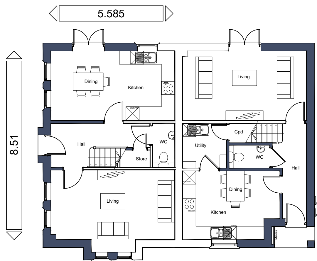
Ground Floor Plan Chepstow Plot 127 Rockfield Plot 128
