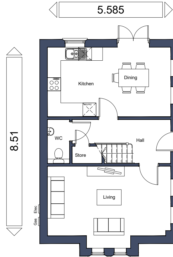
Ground Floor Plan As Plots 18, 25, 68, 92, 94, 99, 139, 148, 177
