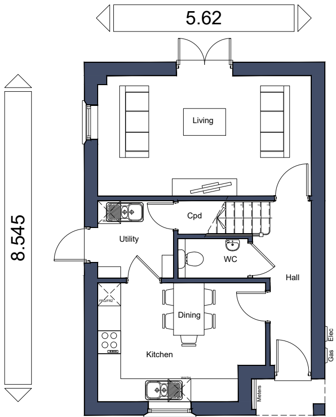
Ground Floor Plan As Plots 83, 90, 124, 128, 150
