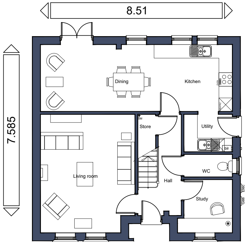
Ground Floor Plan Opp Plots 23, 66, 104, 153, 166, 176
