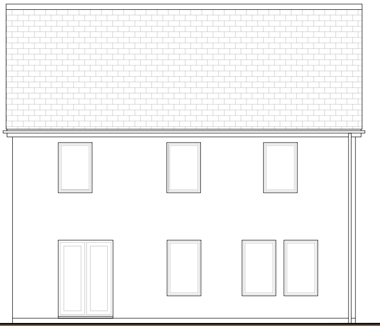
Rear Elevation
