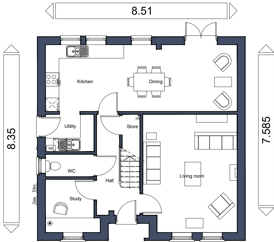
Ground Floor Plan As Plots 1, 17, 24, 70, 76, 159, 185, 187
