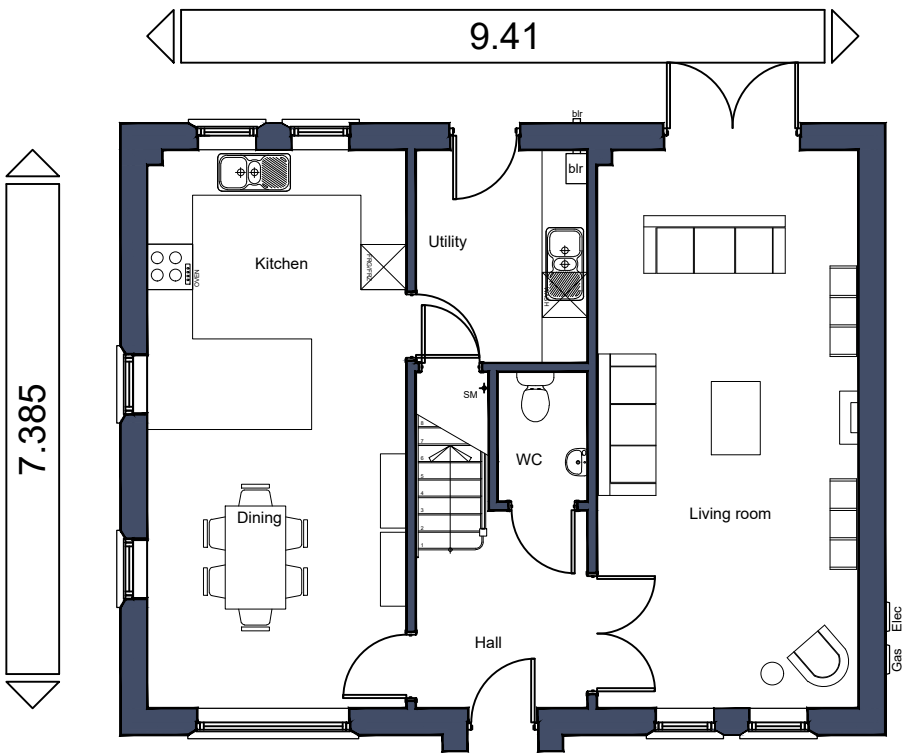
Ground Floor Plan As ( Special) Plot 200
