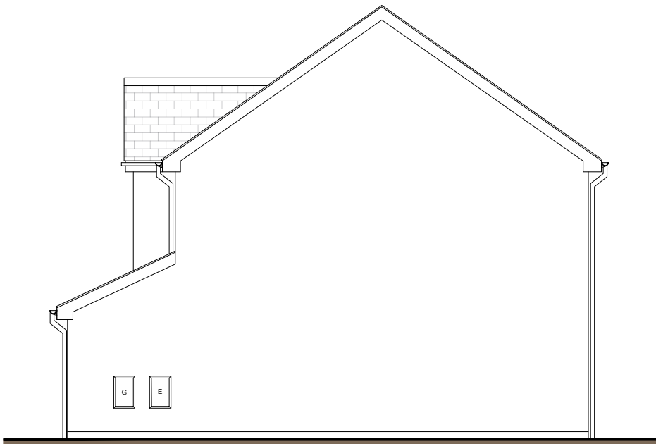
Side Elevation
