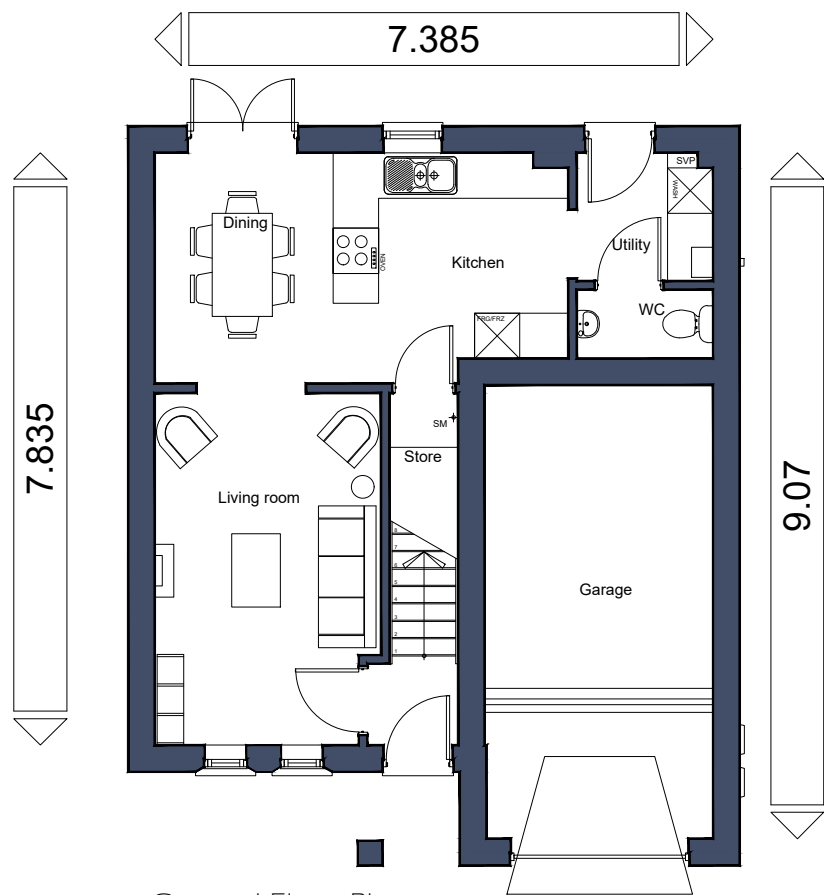
Ground Floor Plan As Plot 170
