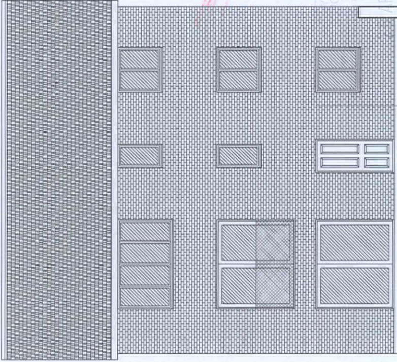
REAR ELEVATION
