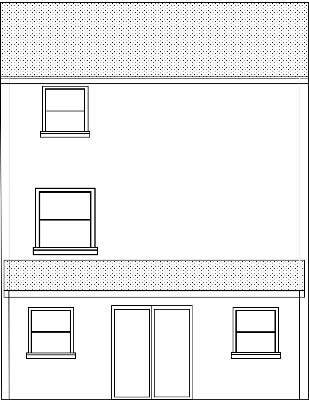
Proposed Rear Elevation - 1:50
