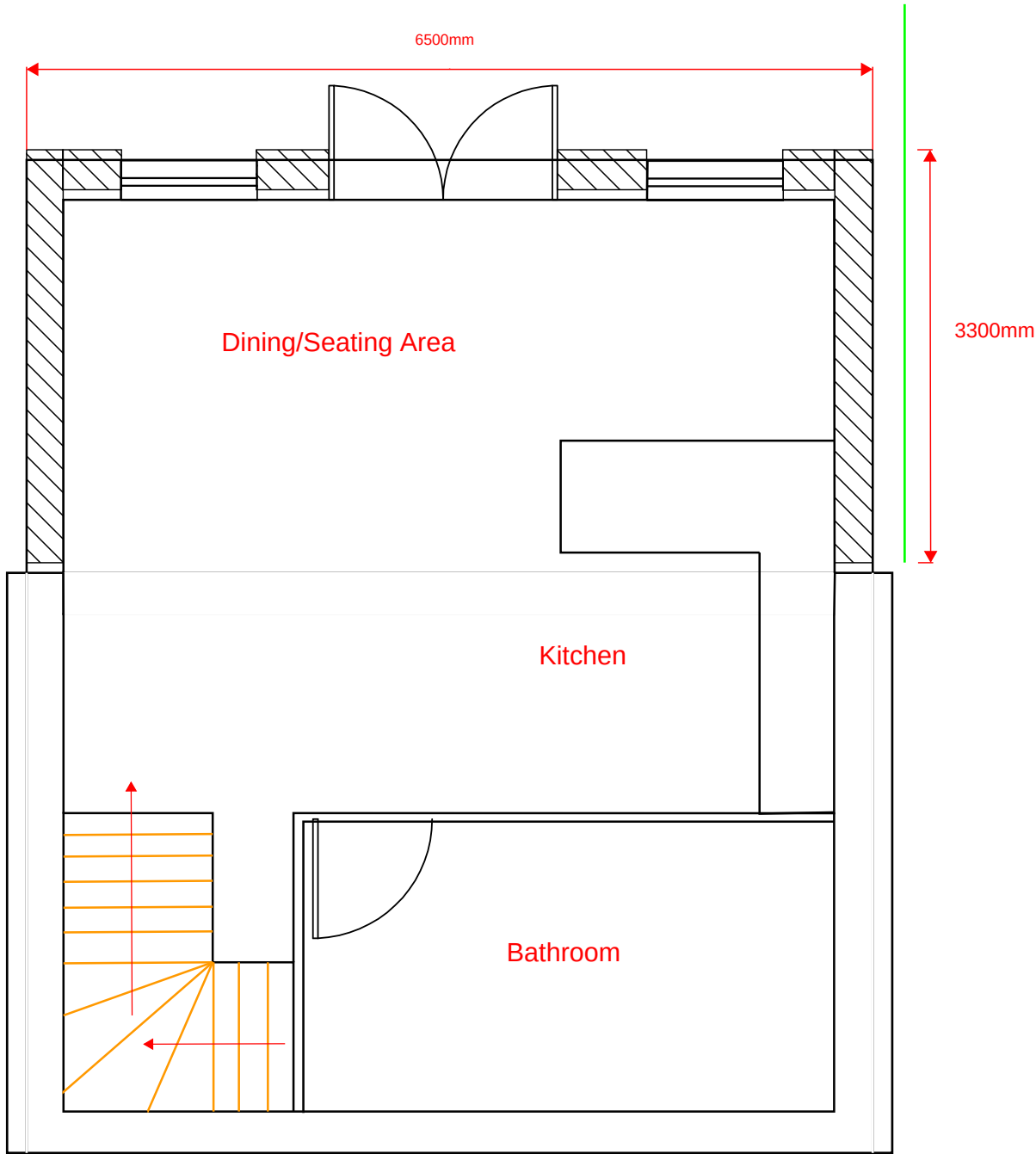
Proposed Lower Ground Floor Plan - 1:50
