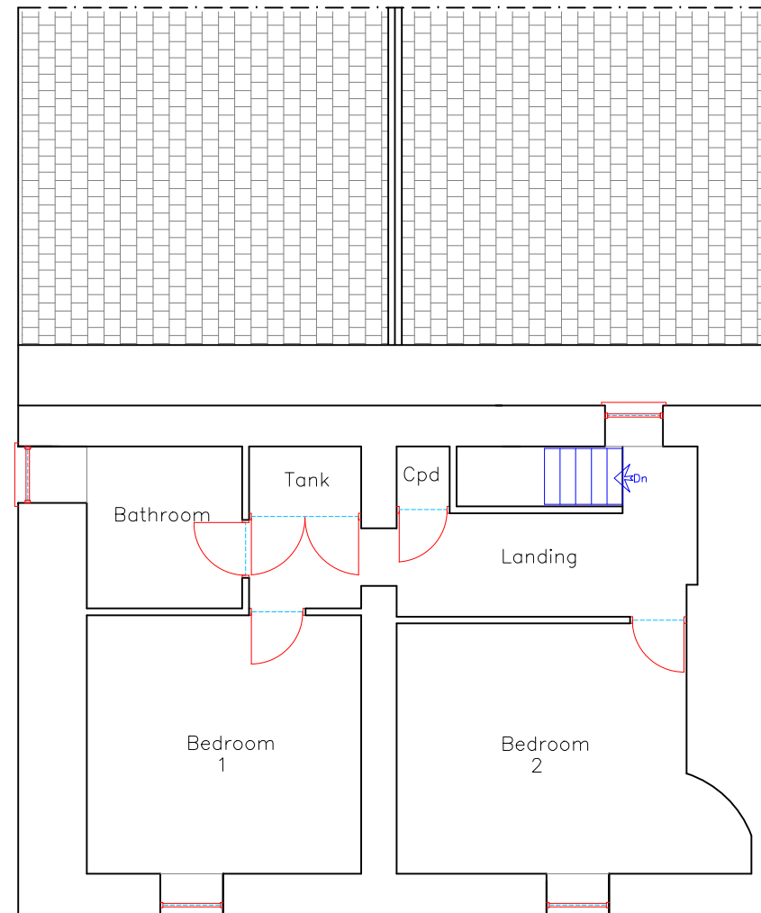
Existing First Floor Plan 1:100
