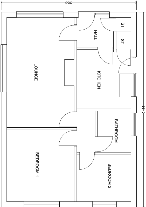
EXISTING PLAN
