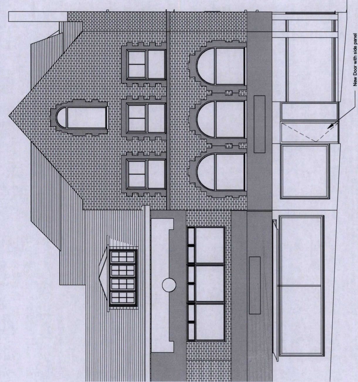
4 Proposed Front Elevation 1 : 100
